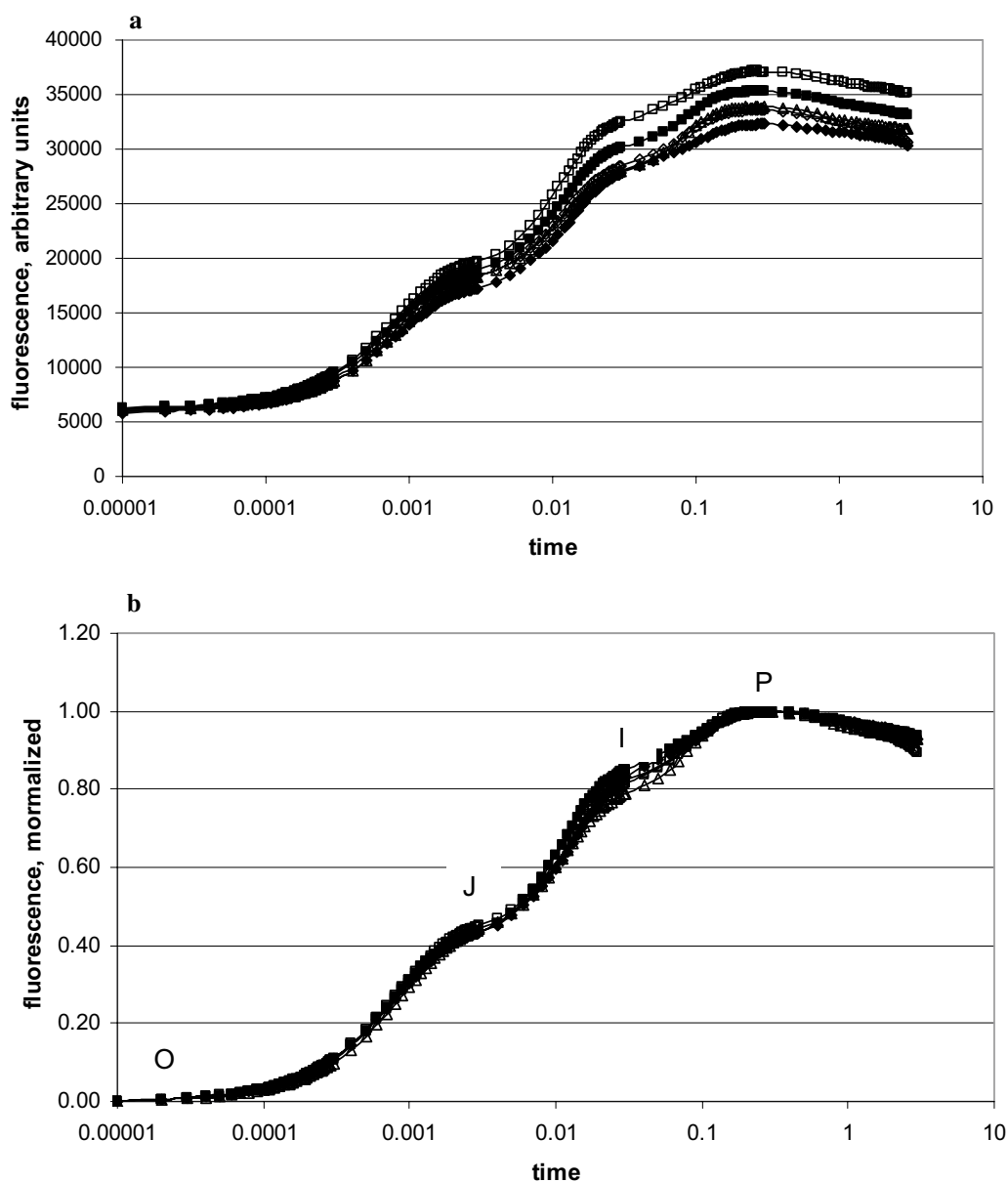
Fig. 5 Fluorescence induction scans from 10 \mu s to 3 s of 5 different Alnus leaves from site b-1, a raw data, b the same data after double normalization between F_o=0 and F_{max} at 0.3 s = 1. All data points are means of 15 measurements (data of 2. August 2017)
