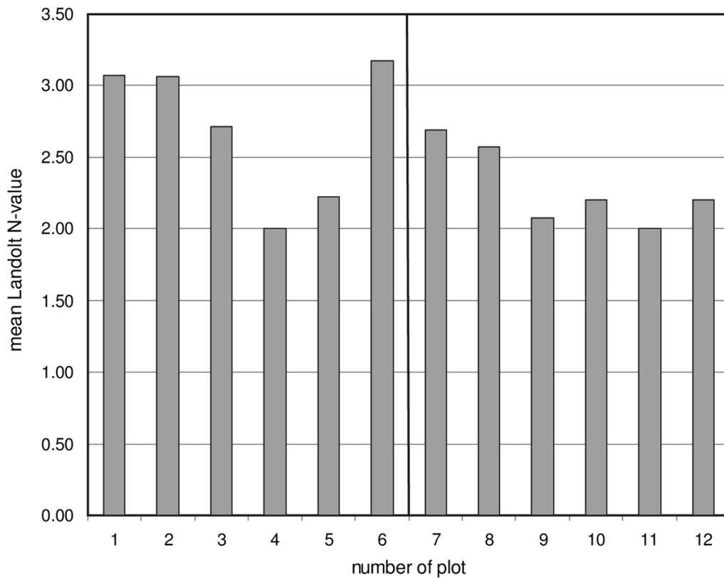
Fig. 3 Mean of indicator values calculated from plant frequency [1] and Landolt indicator value [17] for the 12 sampling plots in the horizontal (1–6) and the vertical (7–12) transects (see Fig. 2)
