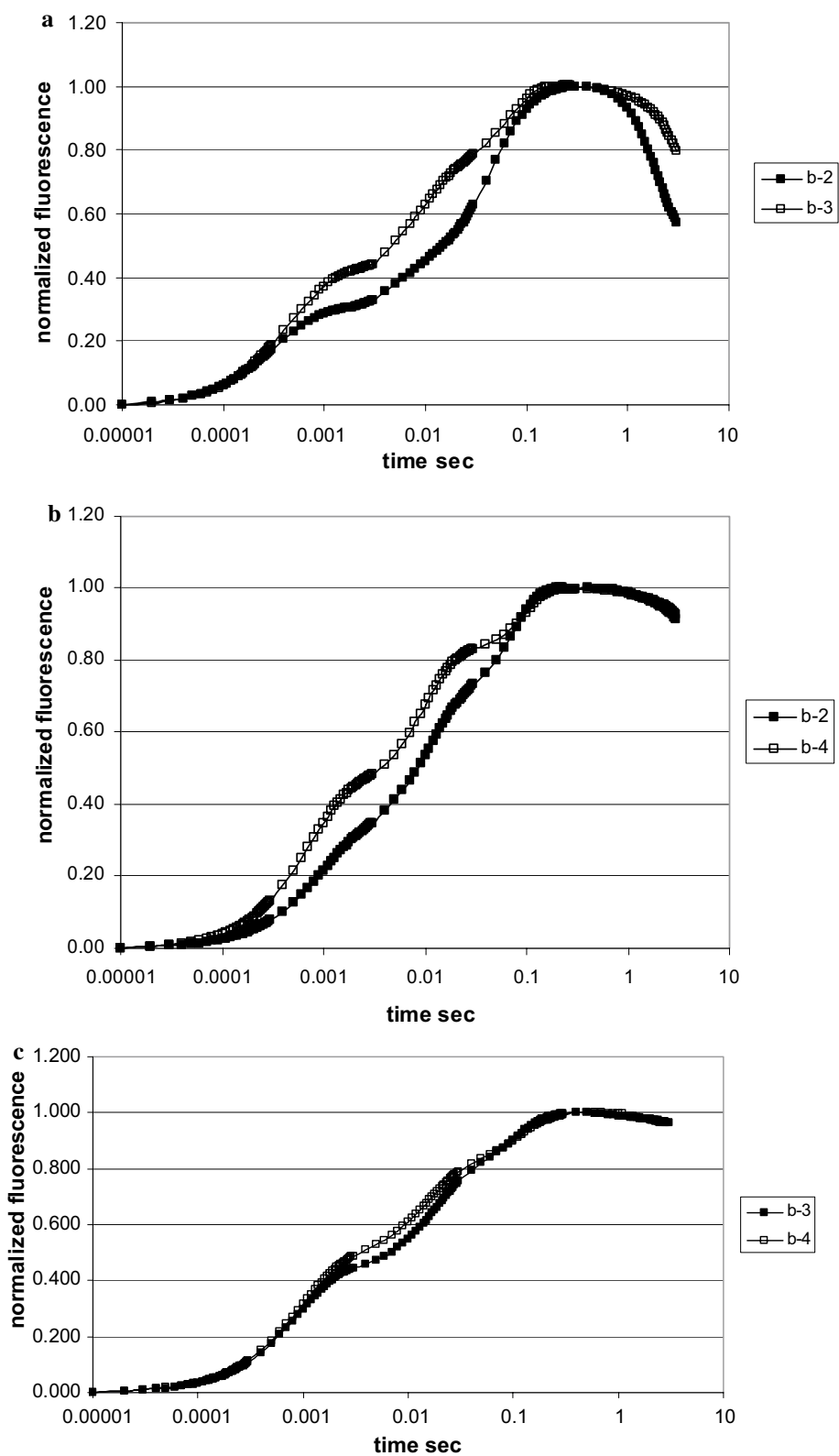
Fig. 6 Fluorescence induction scans from 10 \mu s to 3 s after double normalization between F_o = 0 and F_{max} at 0.3 s = 1, for Calamagrostis (sites b-2 and b-3), Rhododendron (sites b-2 and b-4) (data of 2. August 2017) and Vaccinium (sites b-3 and b-4) (data of 13. September 2017). All data points are means of 15 measurements
