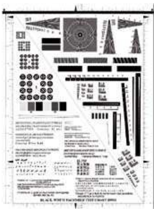
Test Chart No. 4: Black and white facsimile test chart BW01 - (ITU-T Recommendation T.22)
